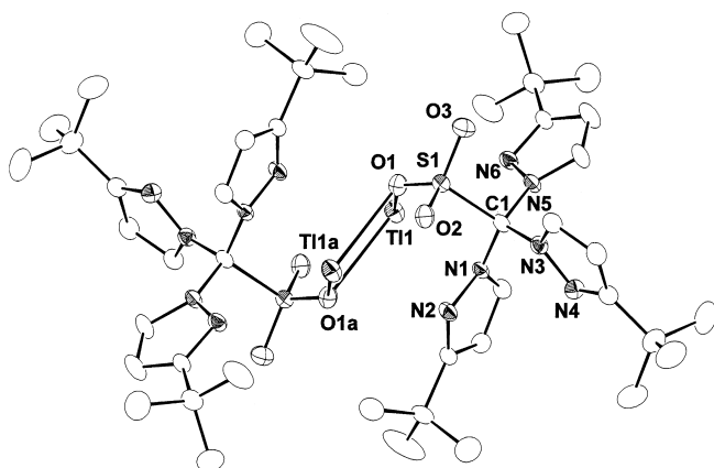
Figure 1. Crystal structure of 2b . Selected distances [Å] and angles [°]: Tl1–O1 2.708(3), Tl1–Tl1a 4.1537(3), S1–O3 1.434(3), S1–O2 1.456(3), S1–O1 1.465(3), S1–C1 1.891(4), O1–Tl1a 2.748(3), N1–N2 1.371(4), N1–C1 1.448(5), N3–N4 1.374(5), N3–C1 1.451(5), N5–N6 1.374(5), N5–C1 1.452(5); O1–Tl1–O1a 80.86(10), O1–Tl1–Tl1a 40.79(6), O1a–Tl1–Tl1a 40.07(6), O2–S1–O1 111.72(18), O1–S1–C1 102.71(17), S1–O1–Tl1 100.26(15), S1–O1–Tl1a 135.99(17), Tl1–O1–Tl1a 99.14(10), N1–C1–N3 109.6(3), N1–C1–N5 109.5(3), N3–C1–N5 108.6(3), N1–C1–S1 110.5(2), N3–C1–S1 110.4(3), N5–C1–S1 108.2(3).
